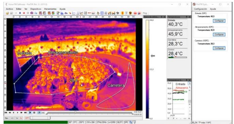
FireTIR software
